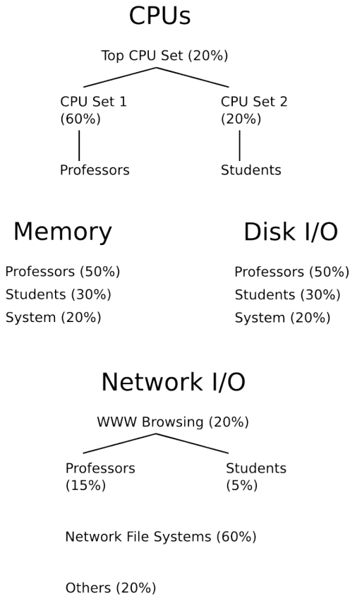
Figure 10.1 Resource Planning
